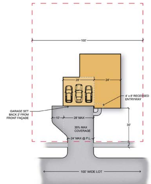
Figure XX - Garage Door Standards - 100' Lot
